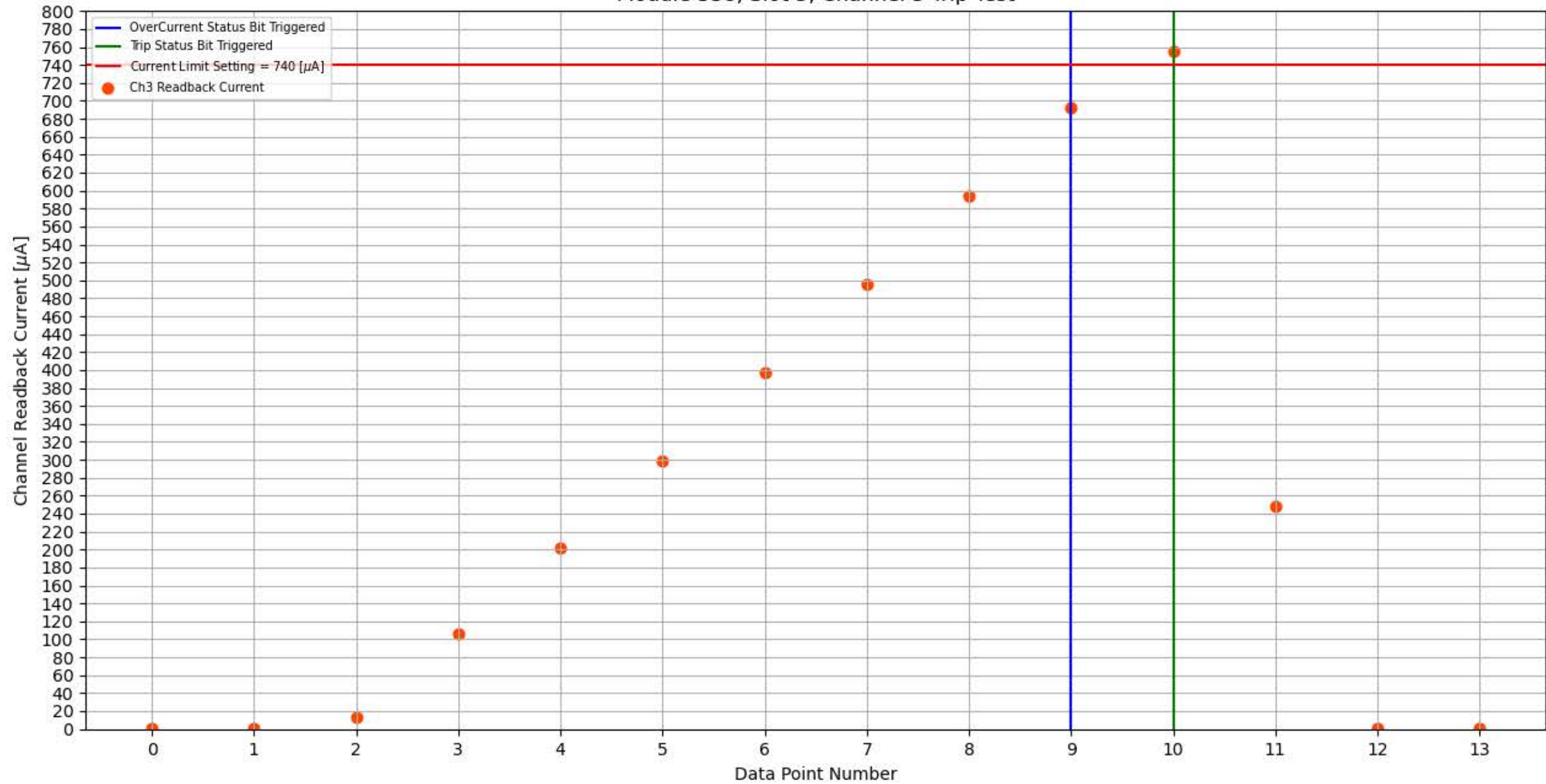
Module 338, Slot 5, Channel 3 Trip Test
