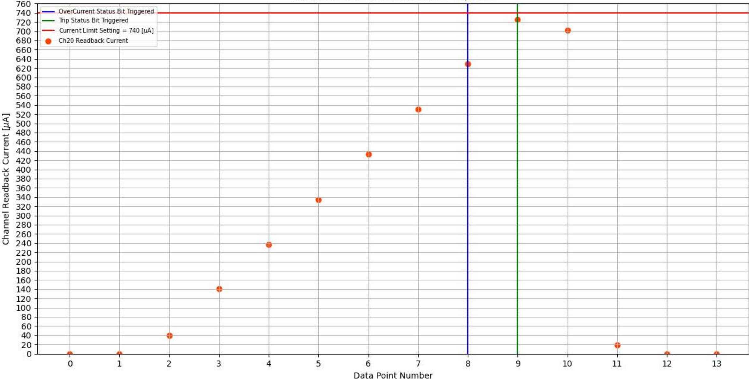
Module 338, Slot 5, Channel 20 Trip Test
