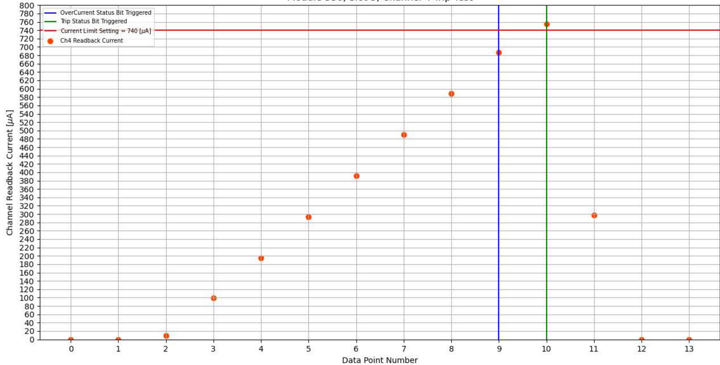
Module 338, Slot 5, Channel 4 Trip Test
