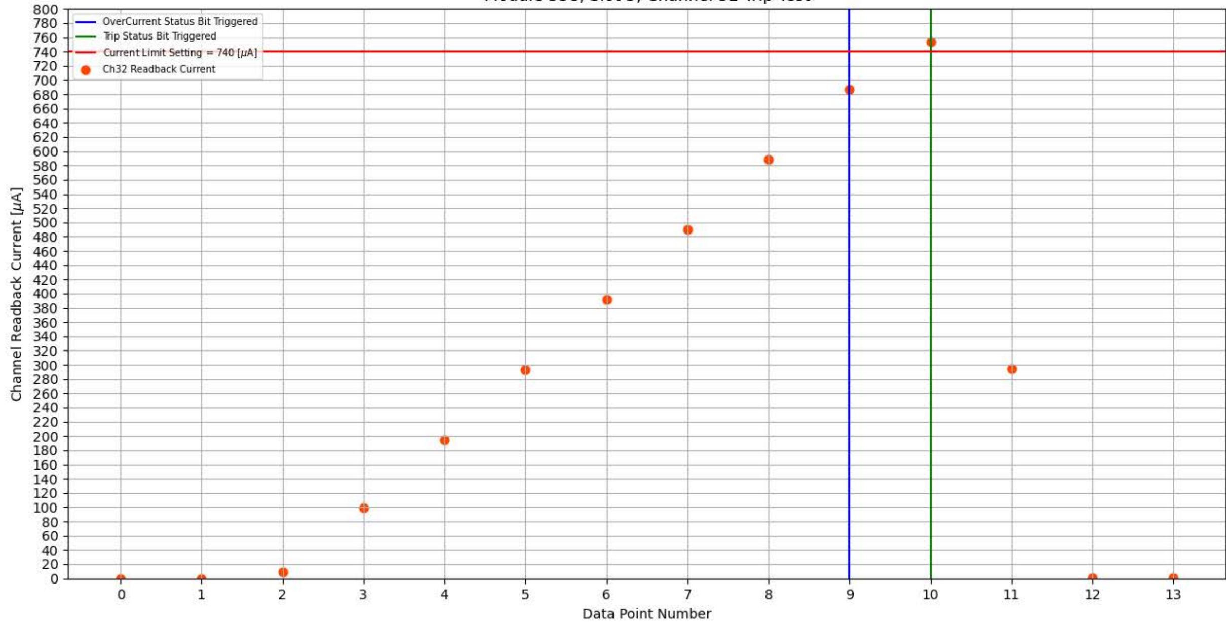
Module 338, Slot 5, Channel 32 Trip Test
