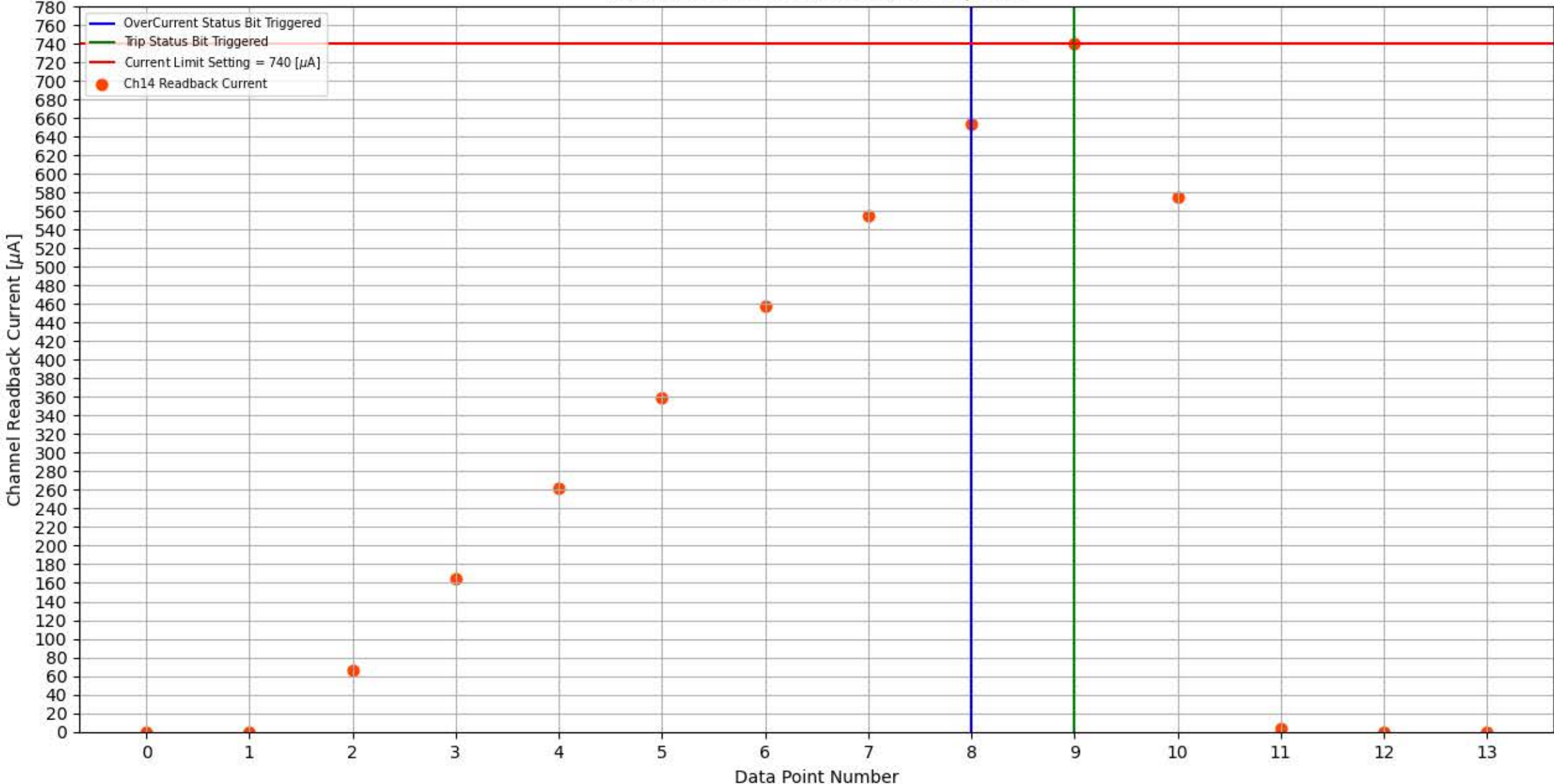
Module 338, Slot 5, Channel 14 Trip Test
