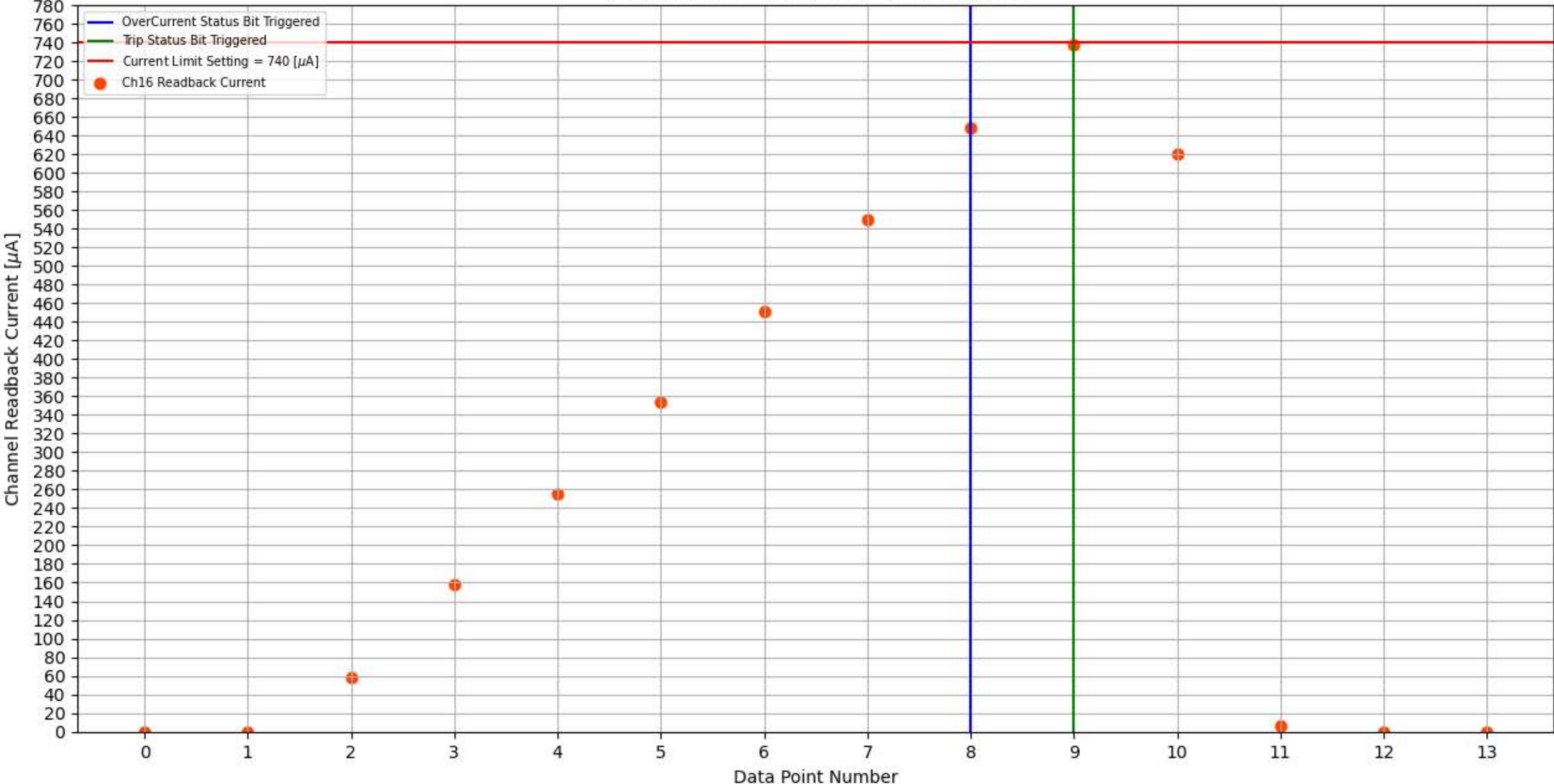
Module 338, Slot 5, Channel 16 Trip Test
