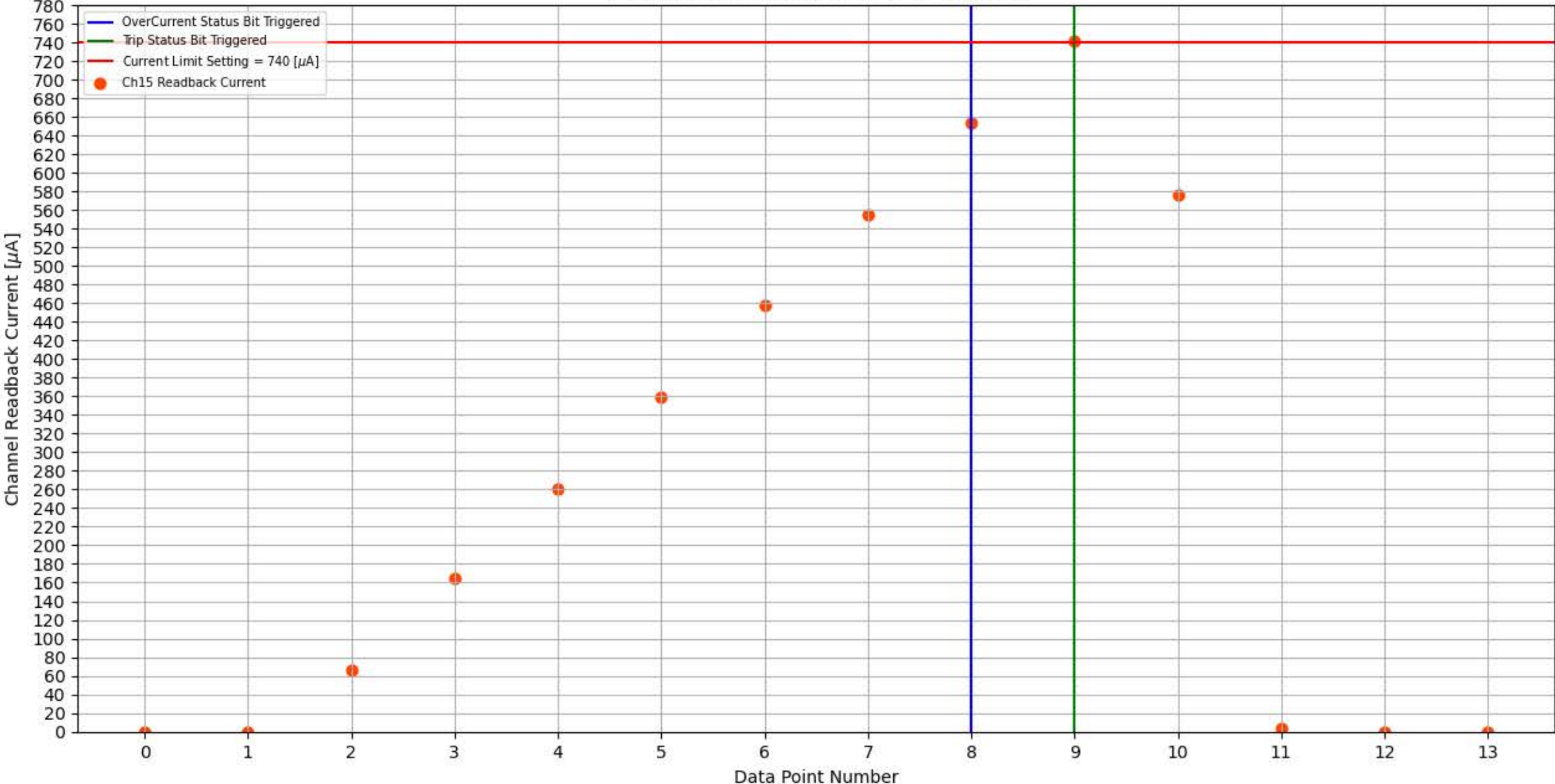
Module 338, Slot 5, Channel 15 Trip Test
