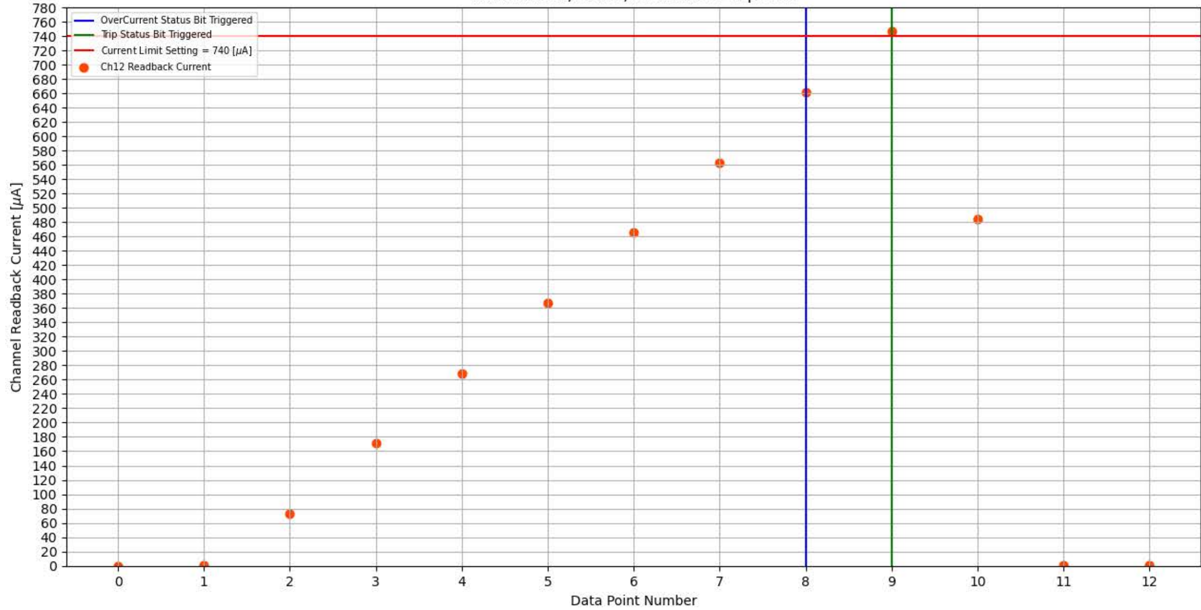
Module 338, Slot 5, Channel 12 Trip Test
