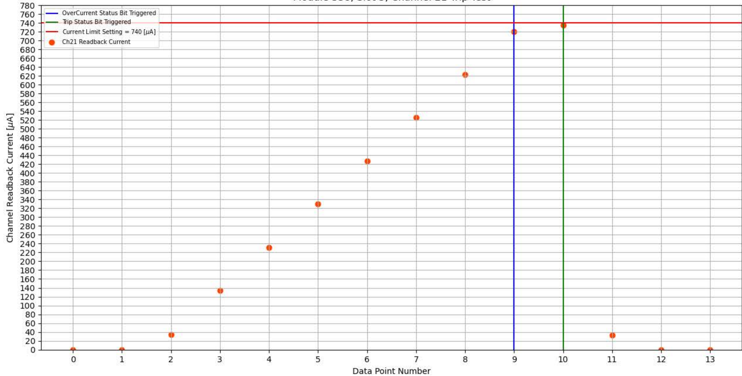
Module 338, Slot 5, Channel 21 Trip Test
