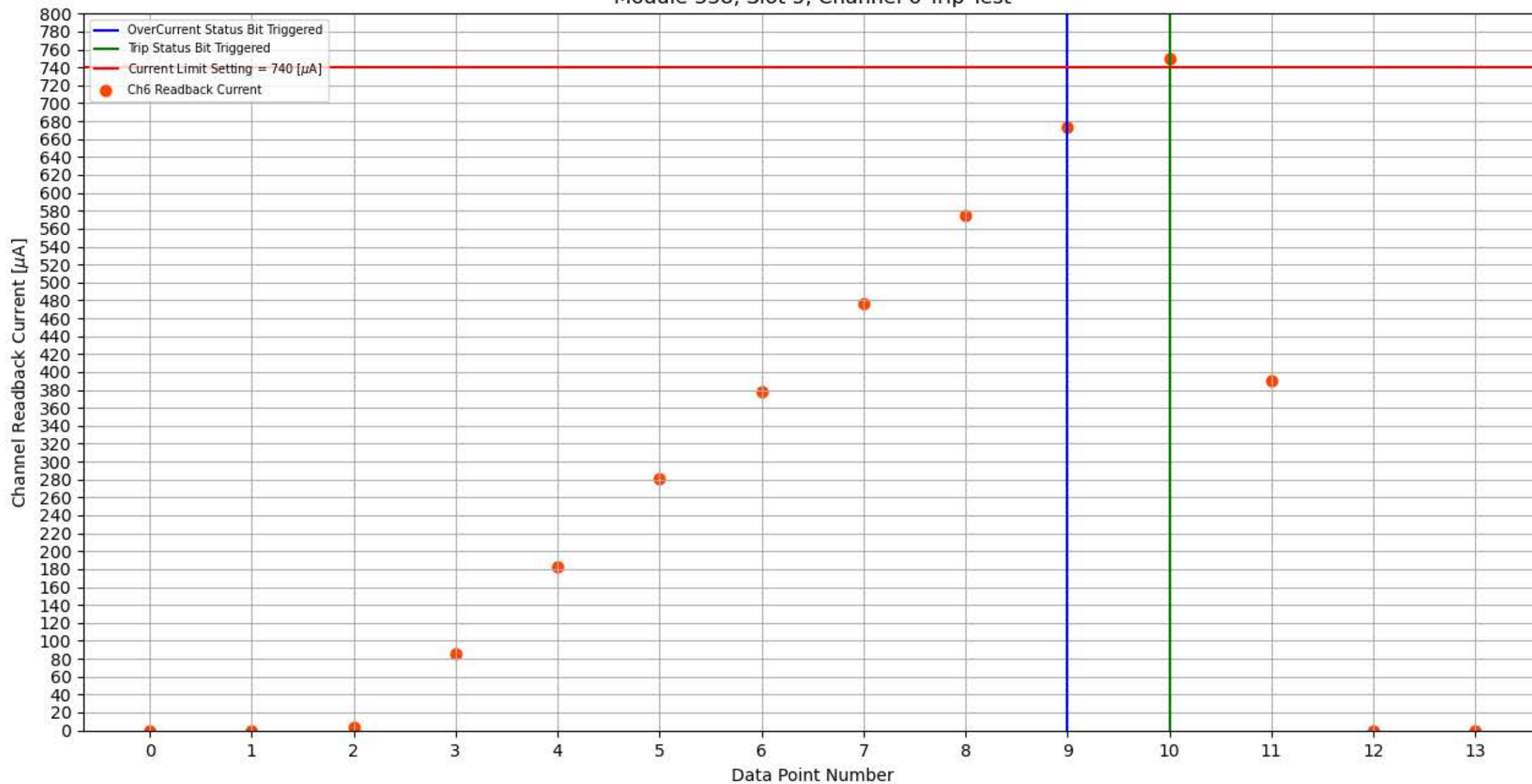
Module 338, Slot 5, Channel 6 Trip Test
