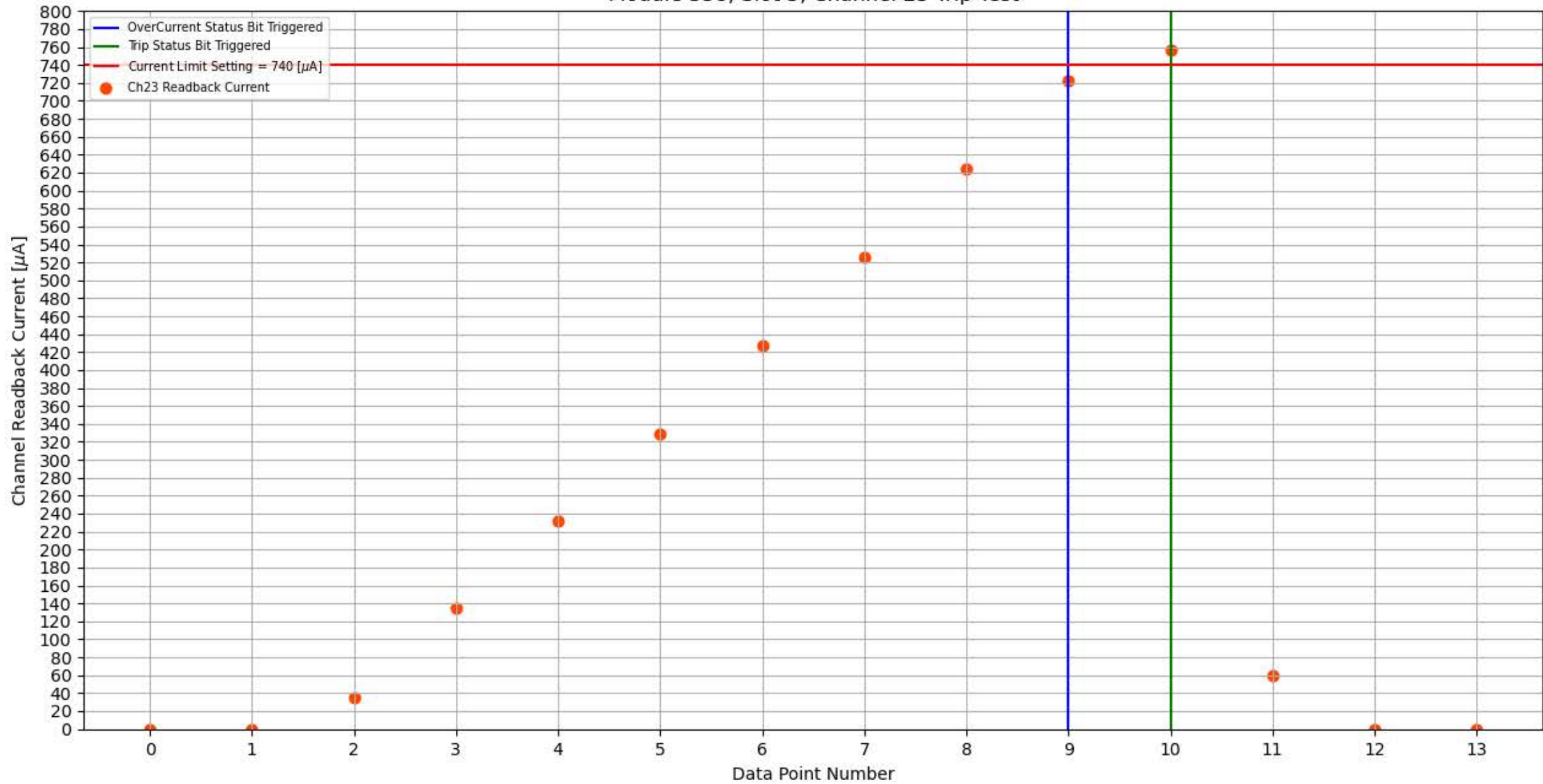
Module 338, Slot 5, Channel 23 Trip Test
