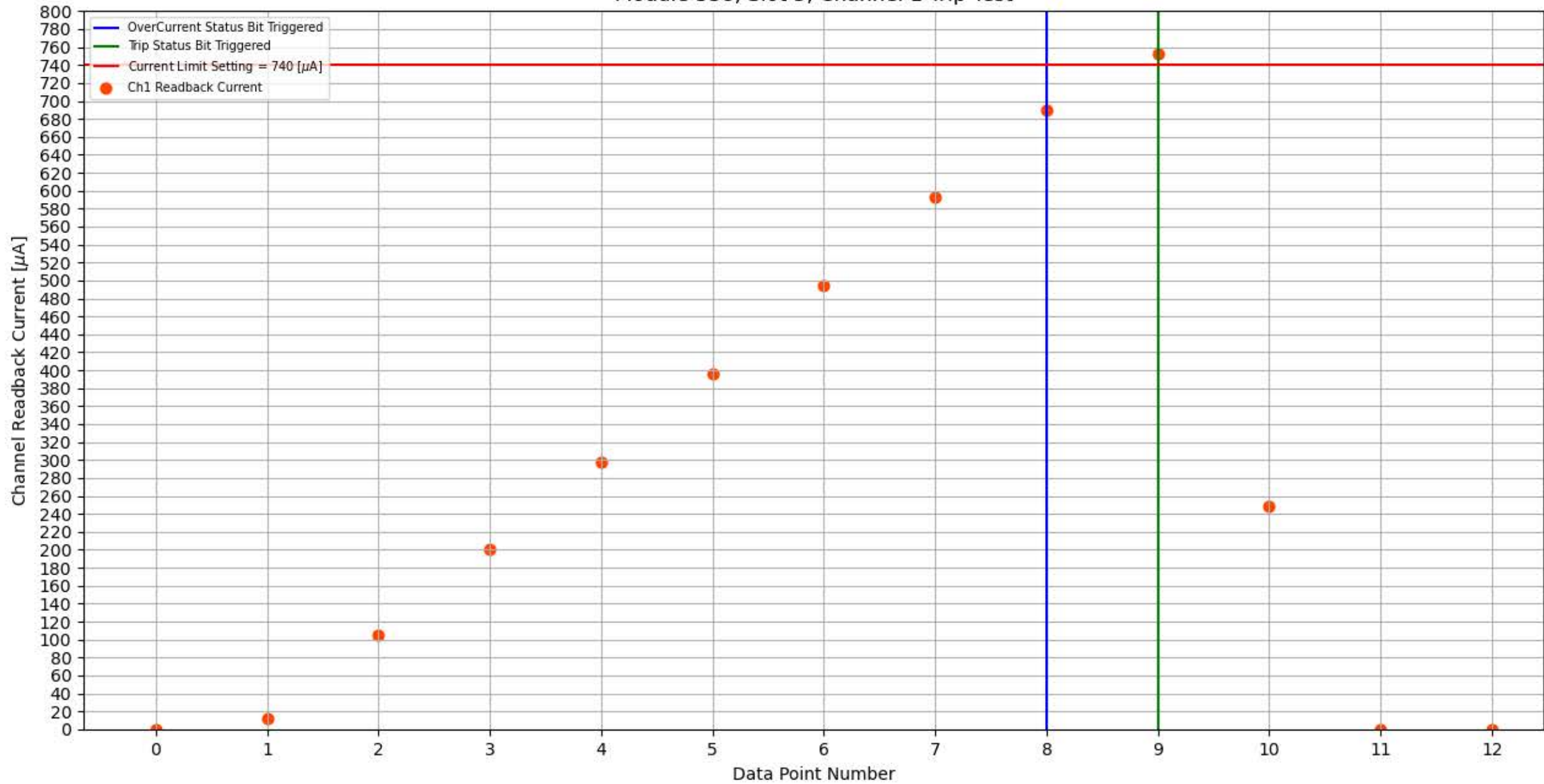
Module 338, Slot 5, Channel 1 Trip Test
