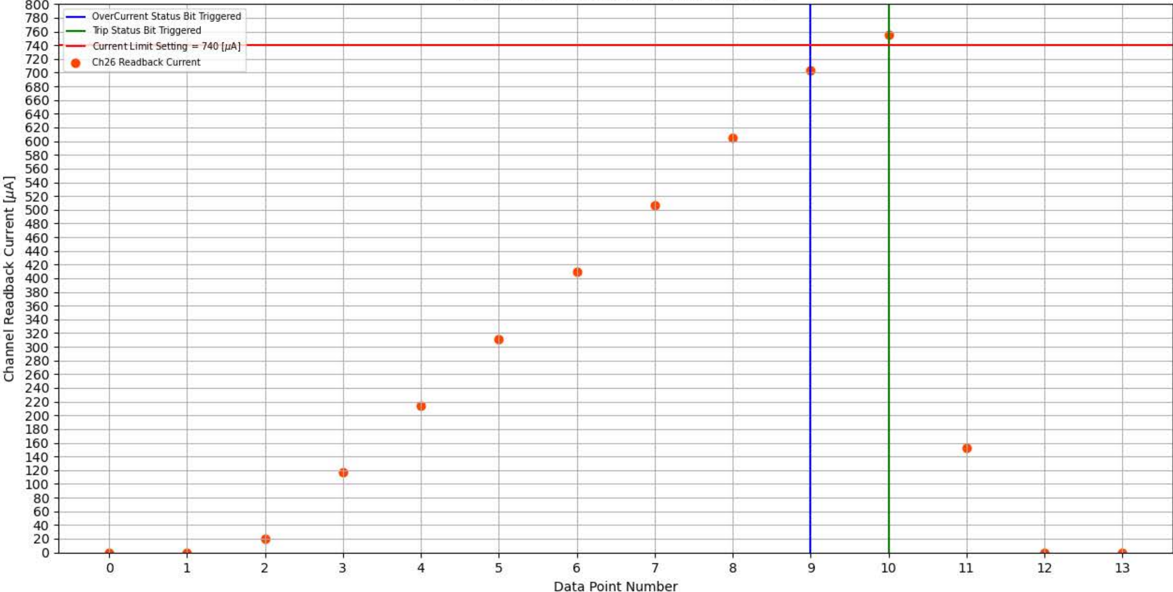
Module 338, Slot 5, Channel 26 Trip Test
