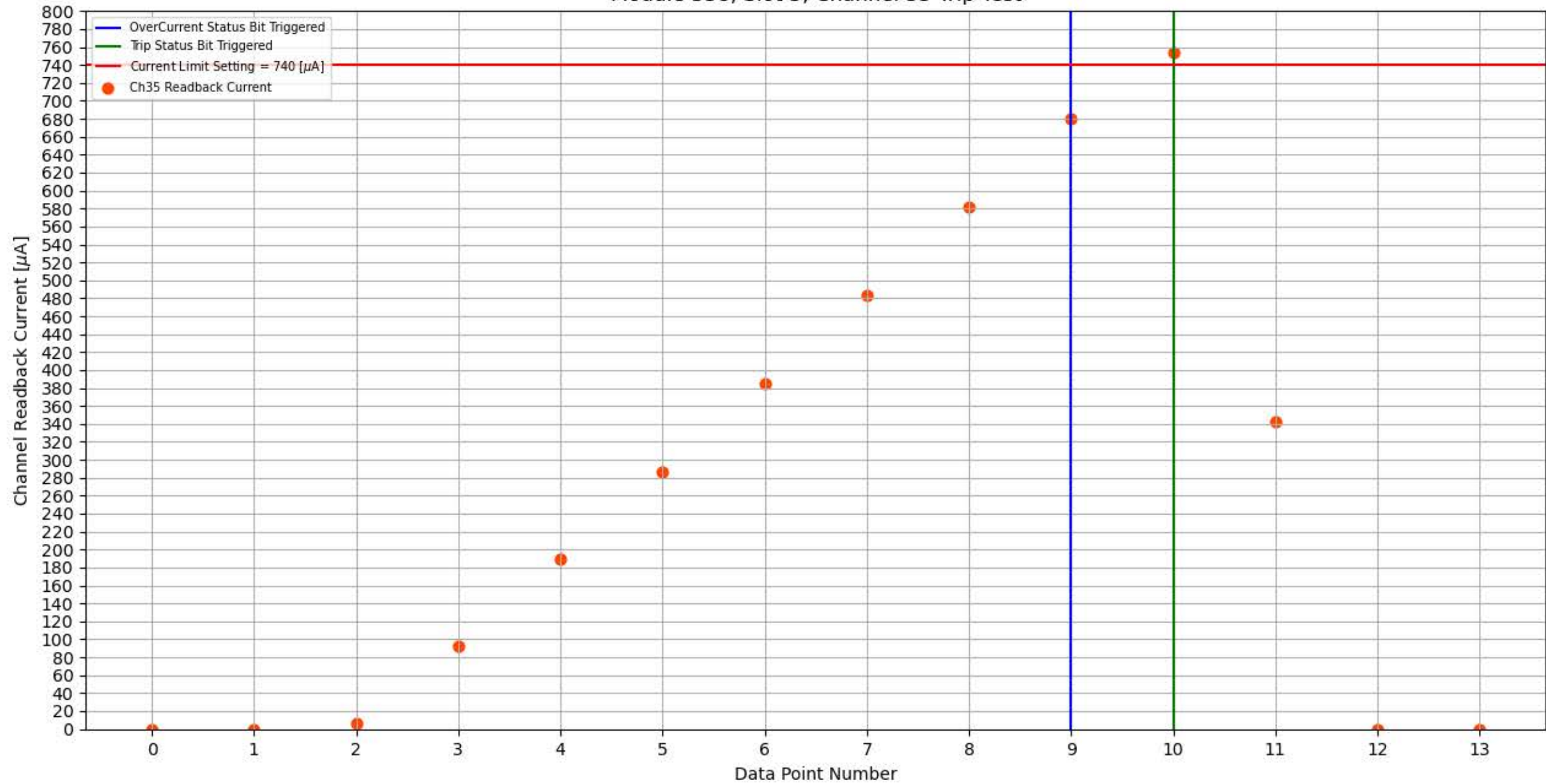
Module 338, Slot 5, Channel 35 Trip Test
