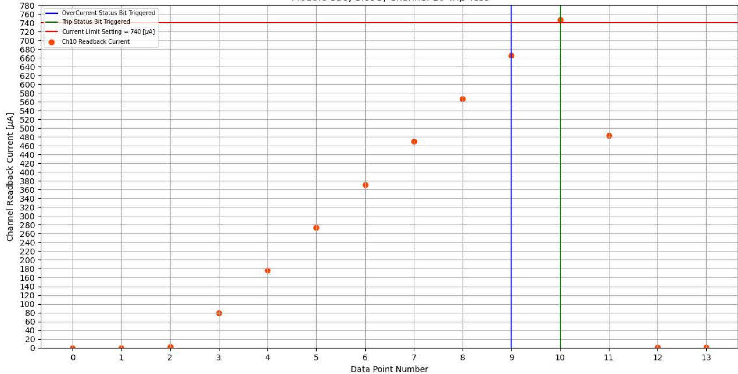
Module 338, Slot 5, Channel 10 Trip Test
