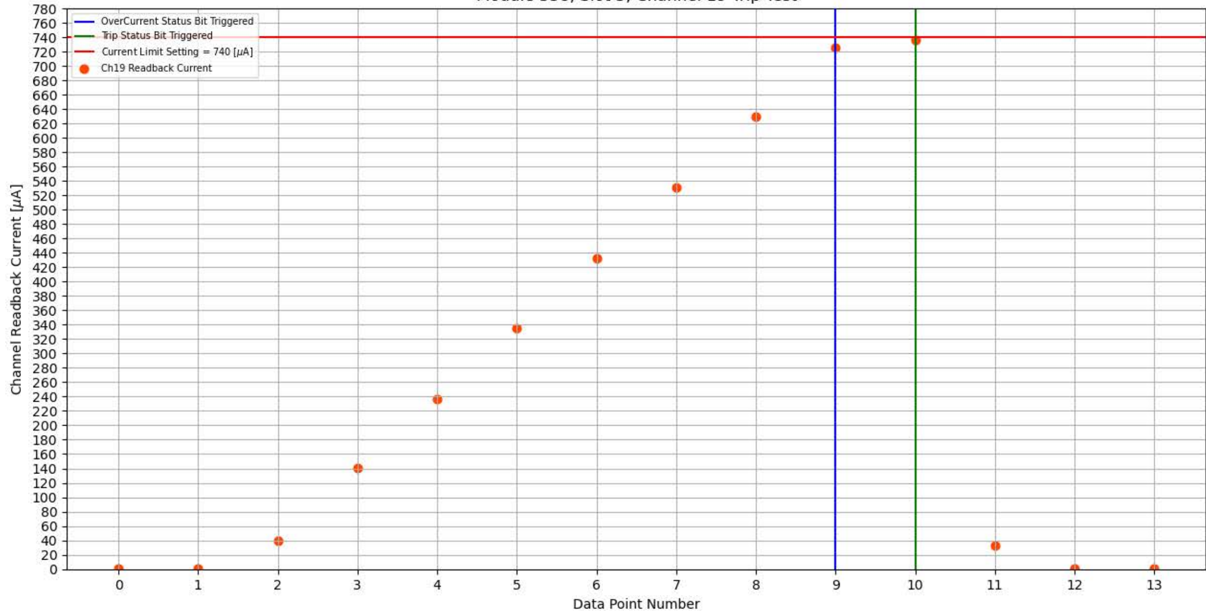
Module 338, Slot 5, Channel 19 Trip Test
