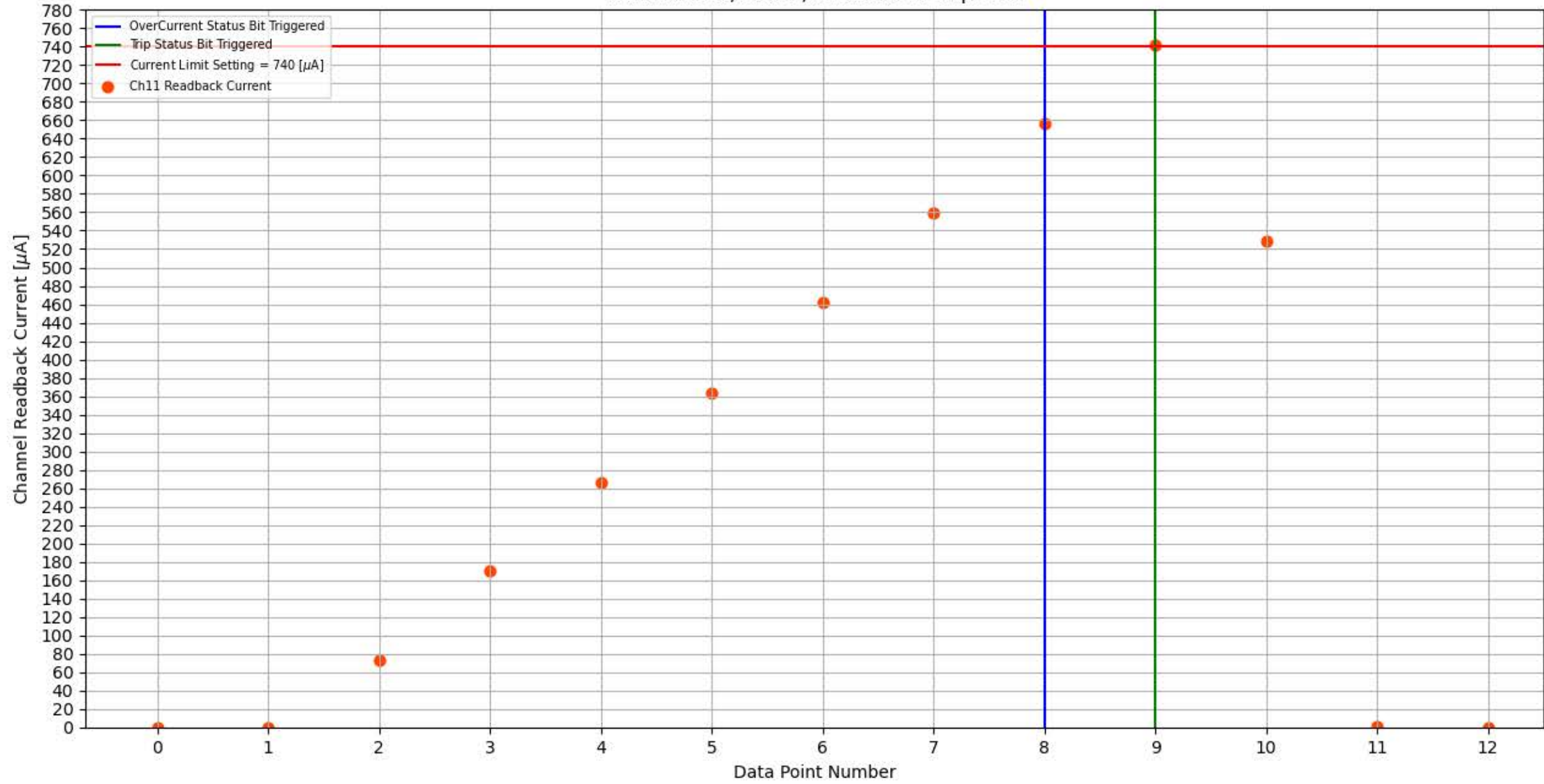
Module 338, Slot 5, Channel 11 Trip Test
