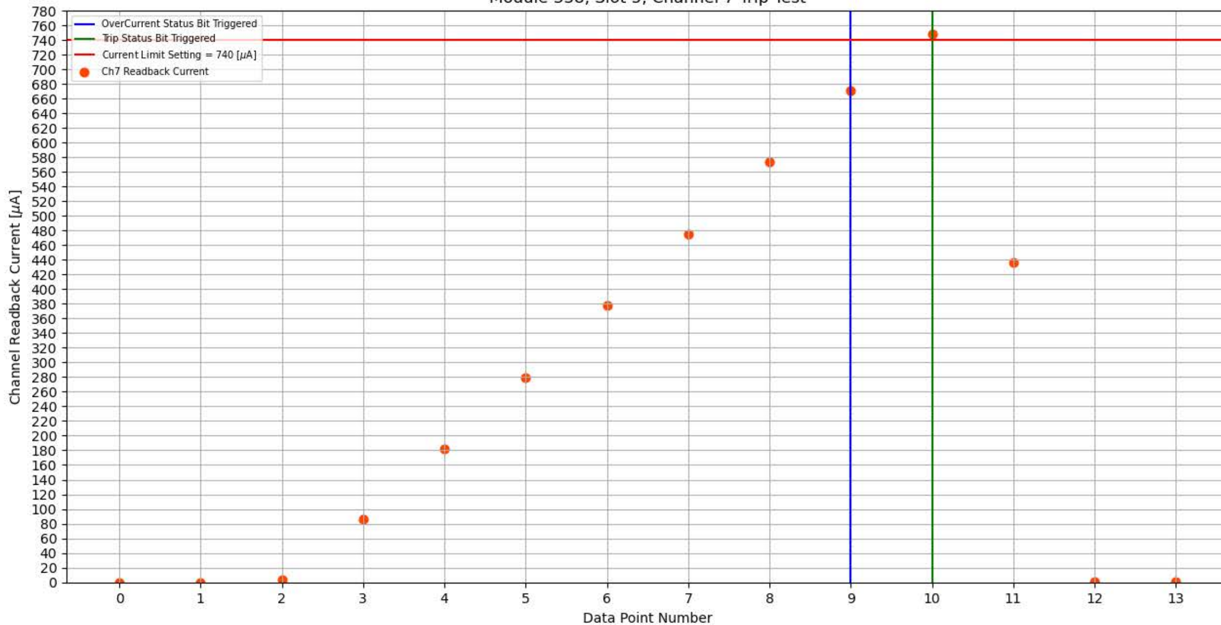
Module 338, Slot 5, Channel 7 Trip Test
