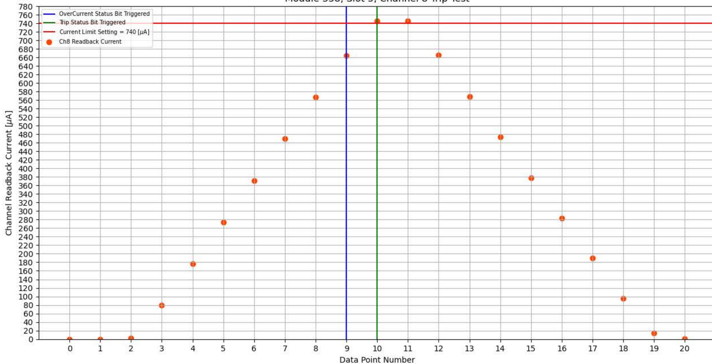
Module 338, Slot 5, Channel 8 Trip Test
