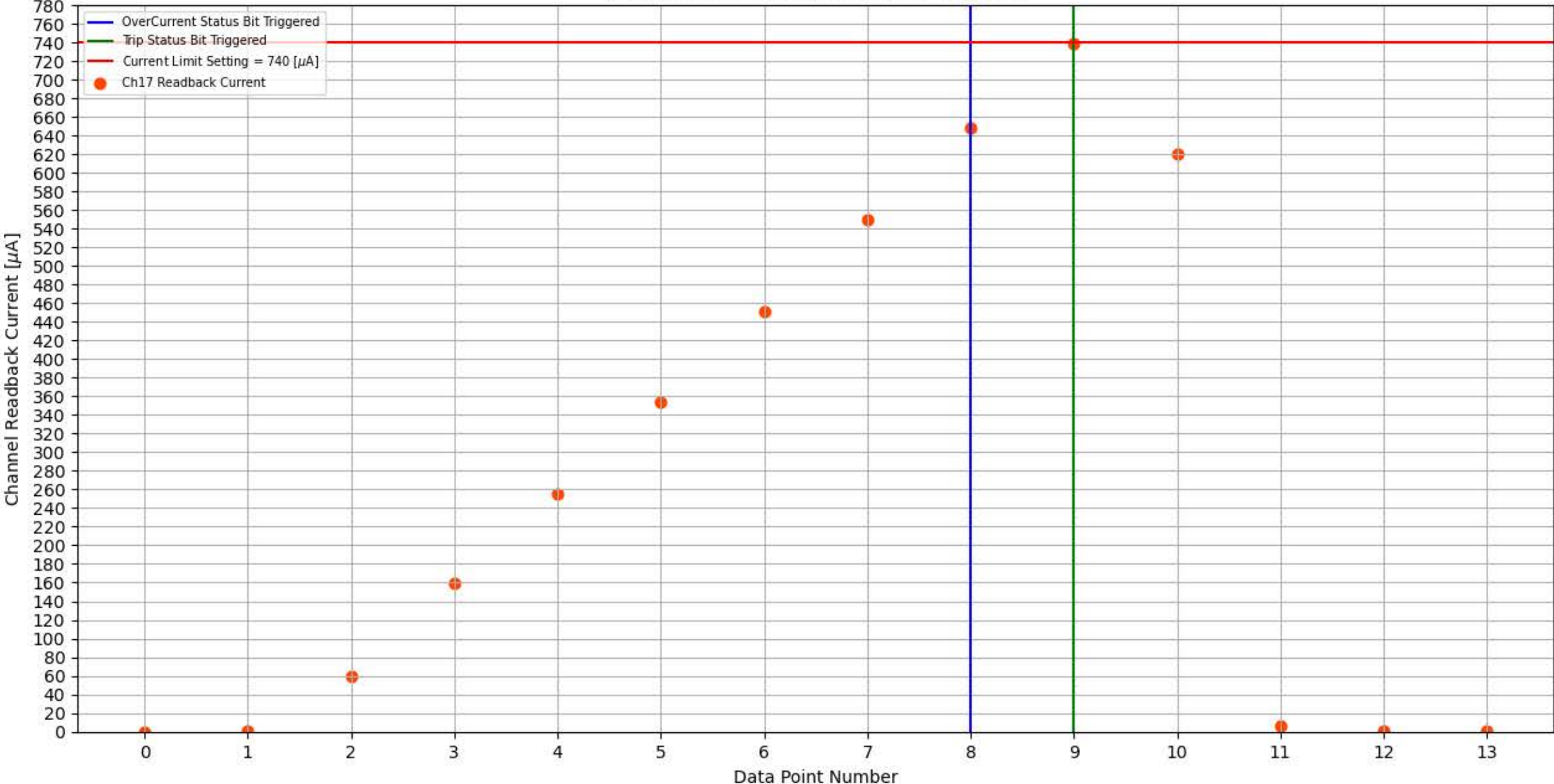
Module 338, Slot 5, Channel 17 Trip Test
