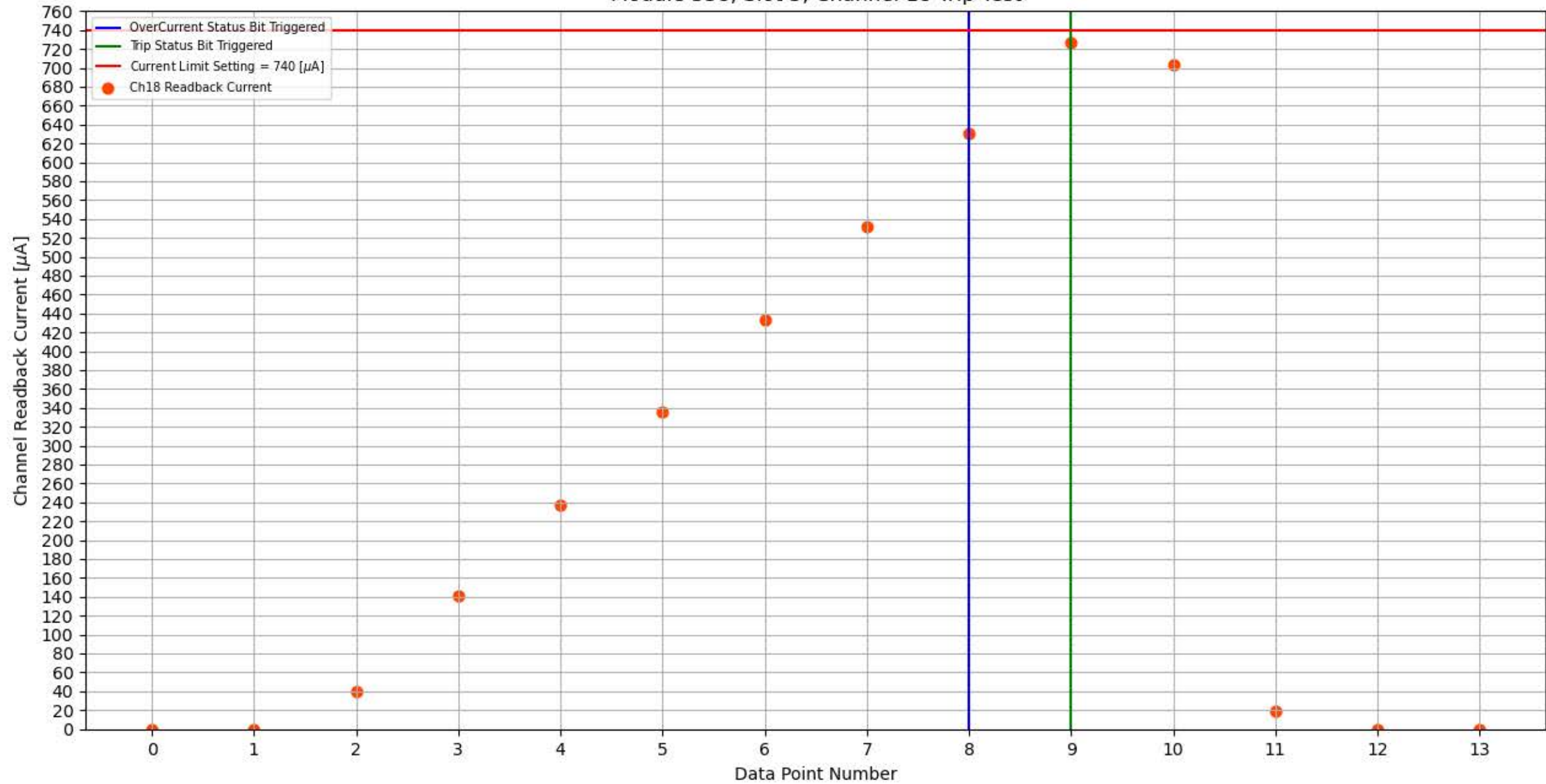
Module 338, Slot 5, Channel 18 Trip Test
