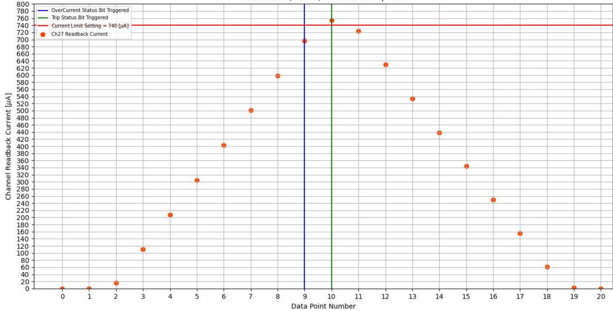
Module 338, Slot 5, Channel 27 Trip Test
