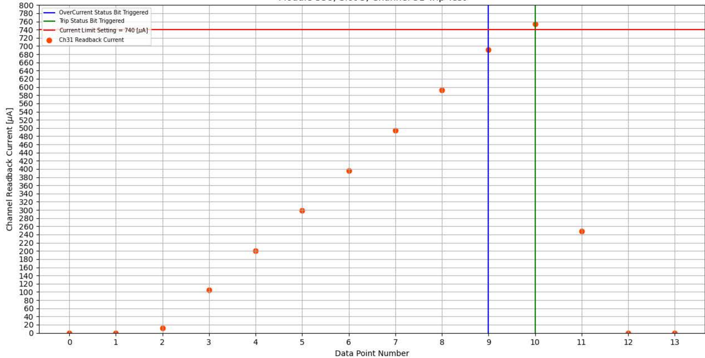
Module 338, Slot 5, Channel 31 Trip Test
