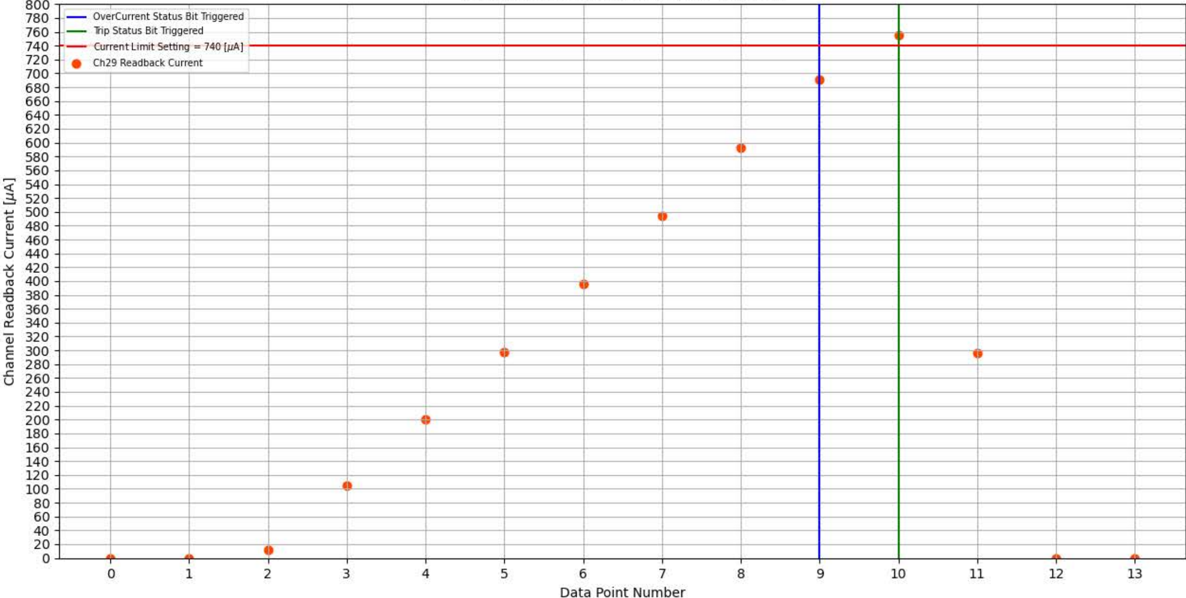
Module 338, Slot 5, Channel 29 Trip Test
