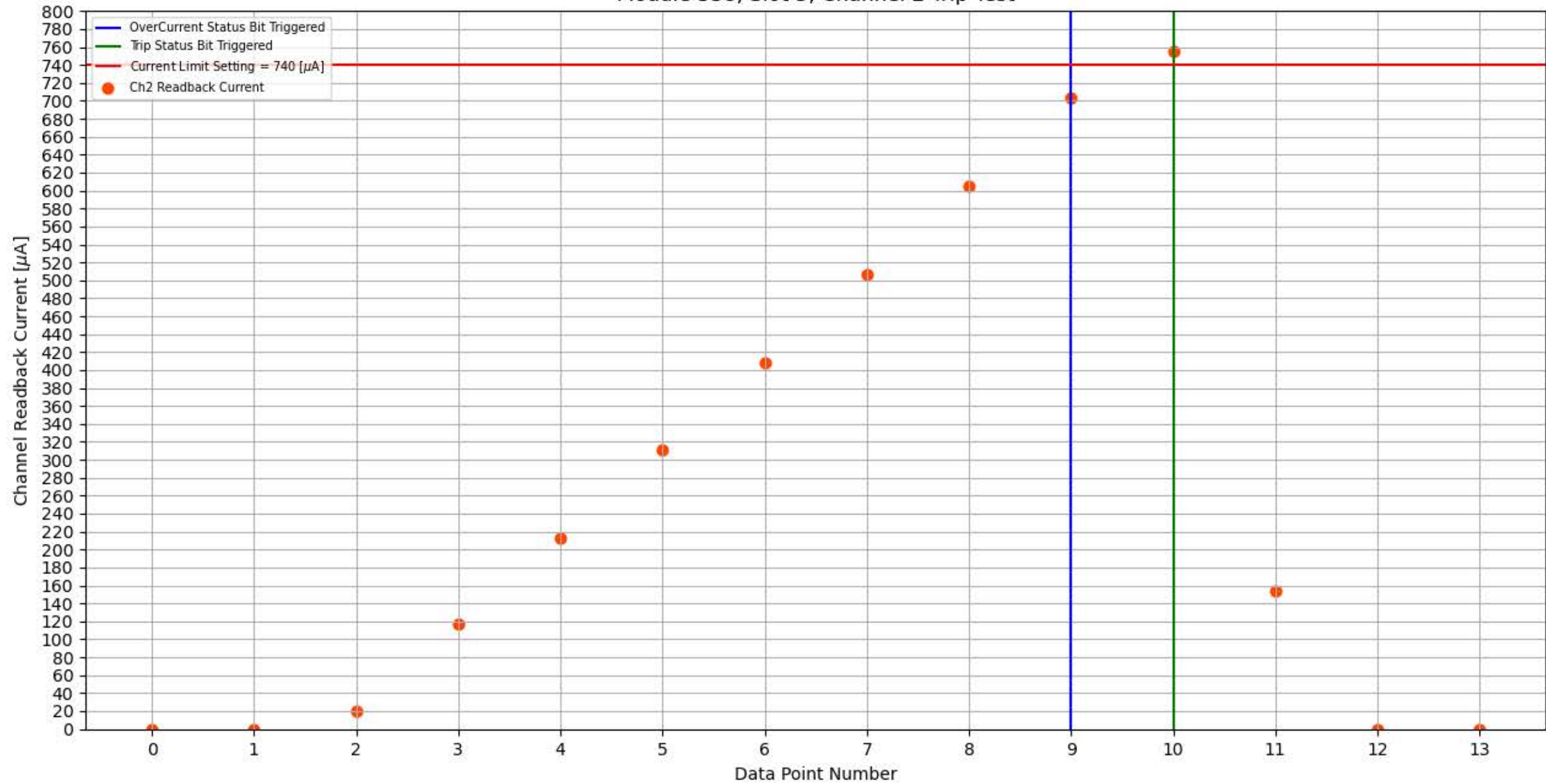
Module 338, Slot 5, Channel 2 Trip Test
