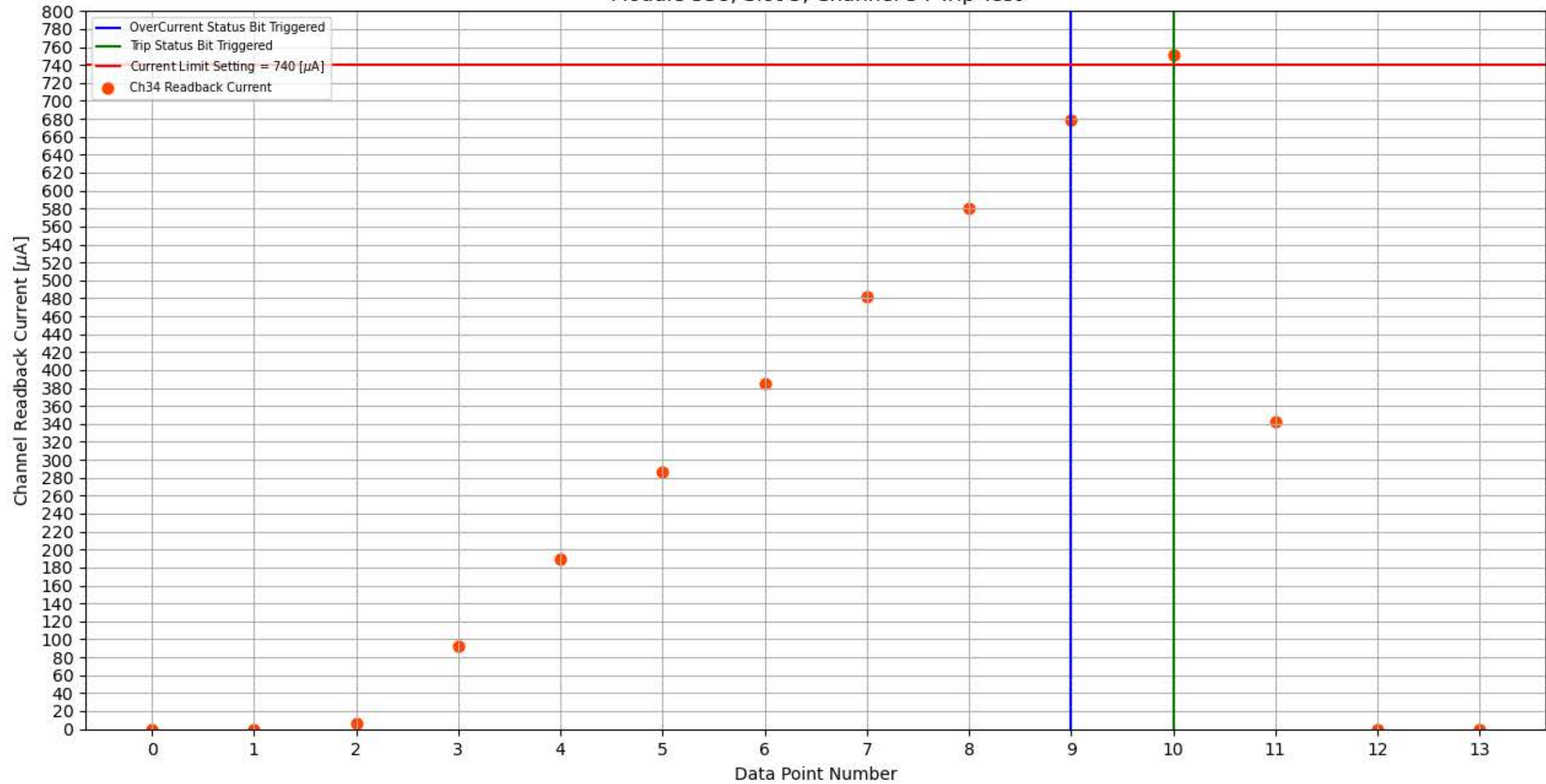
Module 338, Slot 5, Channel 34 Trip Test
