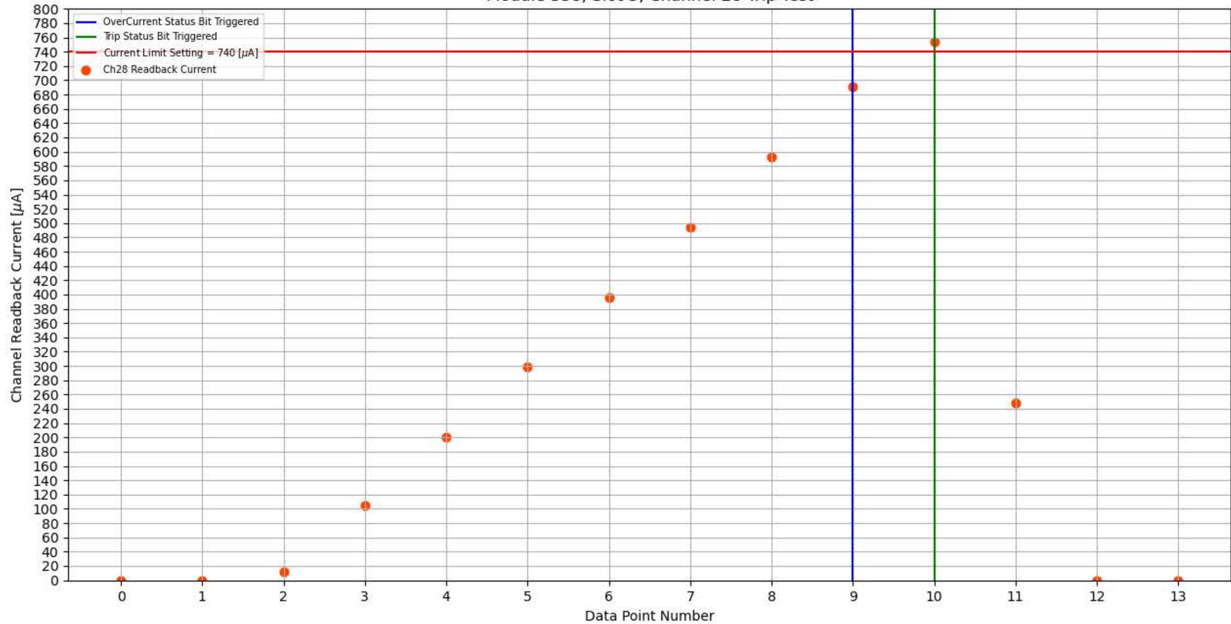
Module 338, Slot 5, Channel 28 Trip Test
