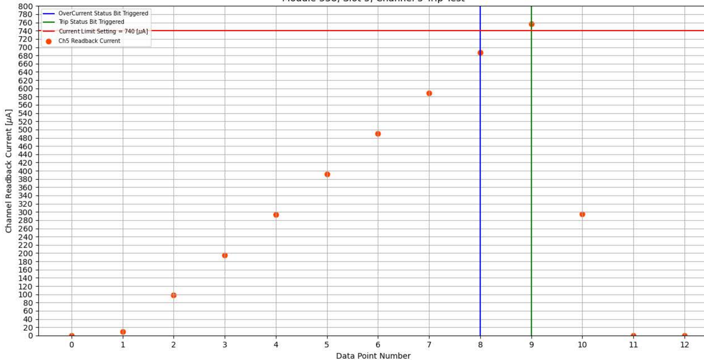
Module 338, Slot 5, Channel 5 Trip Test
