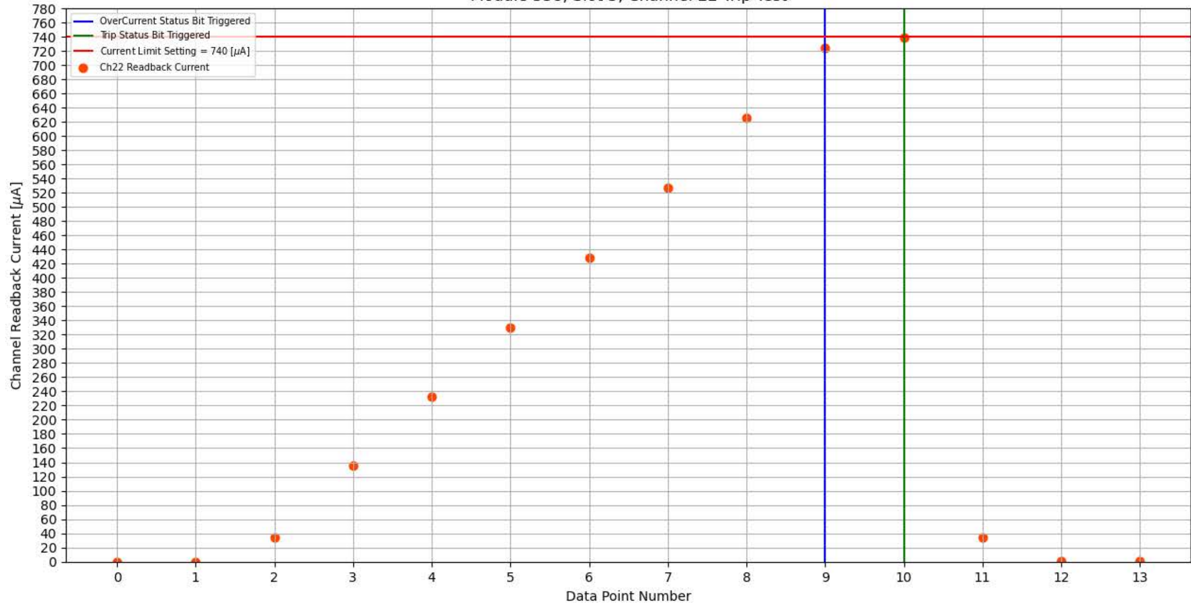
Module 338, Slot 5, Channel 22 Trip Test
