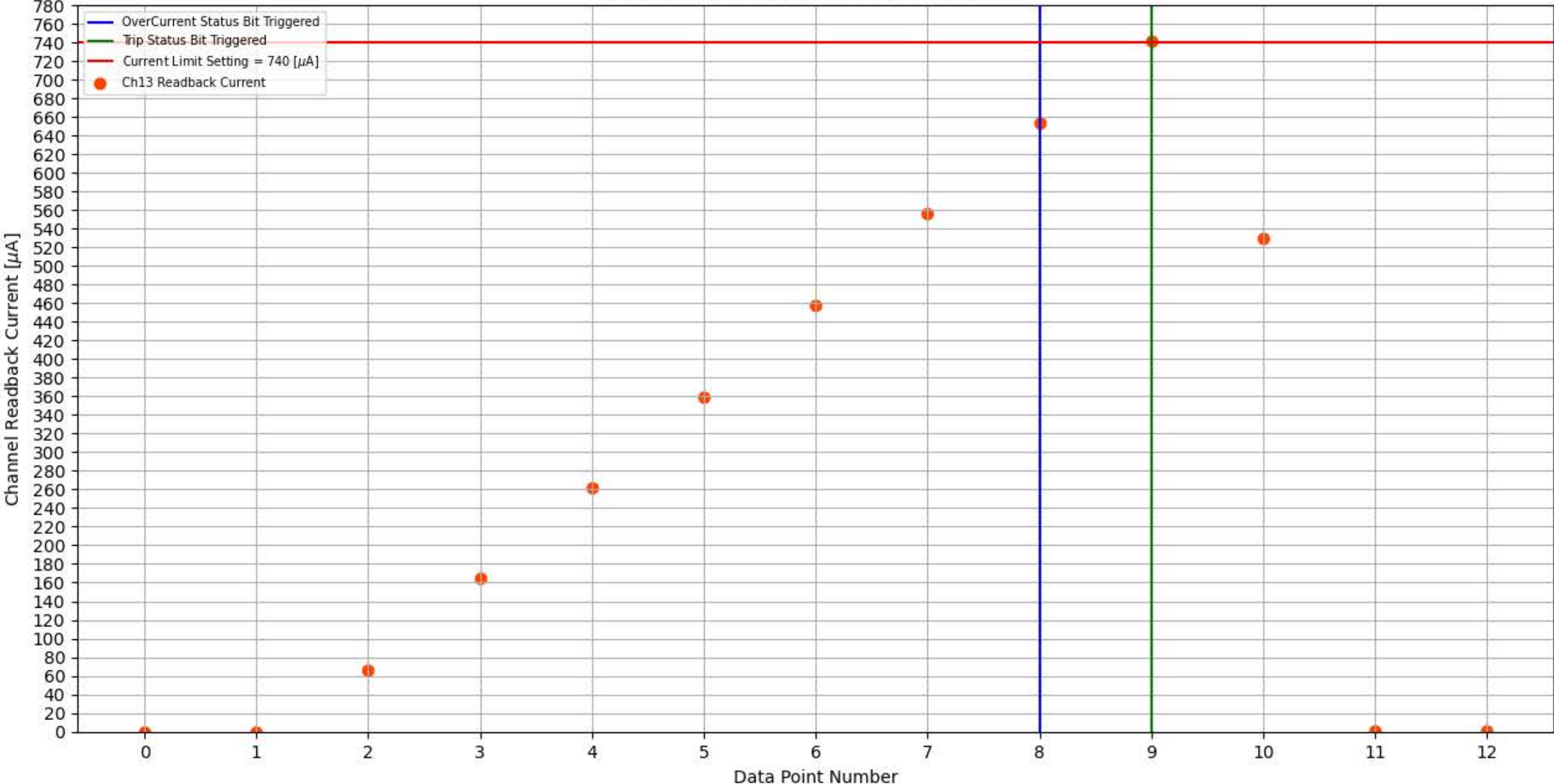
Module 338, Slot 5, Channel 13 Trip Test
