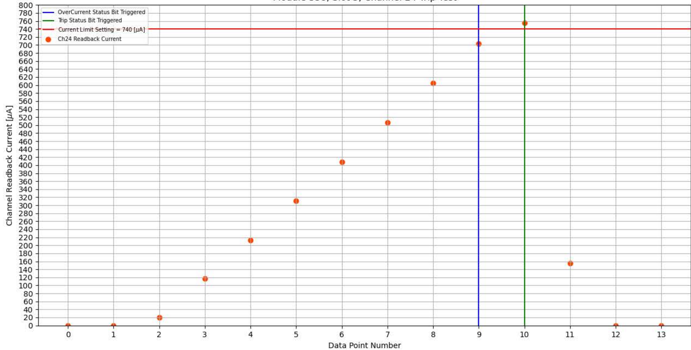
Module 338, Slot 5, Channel 24 Trip Test
