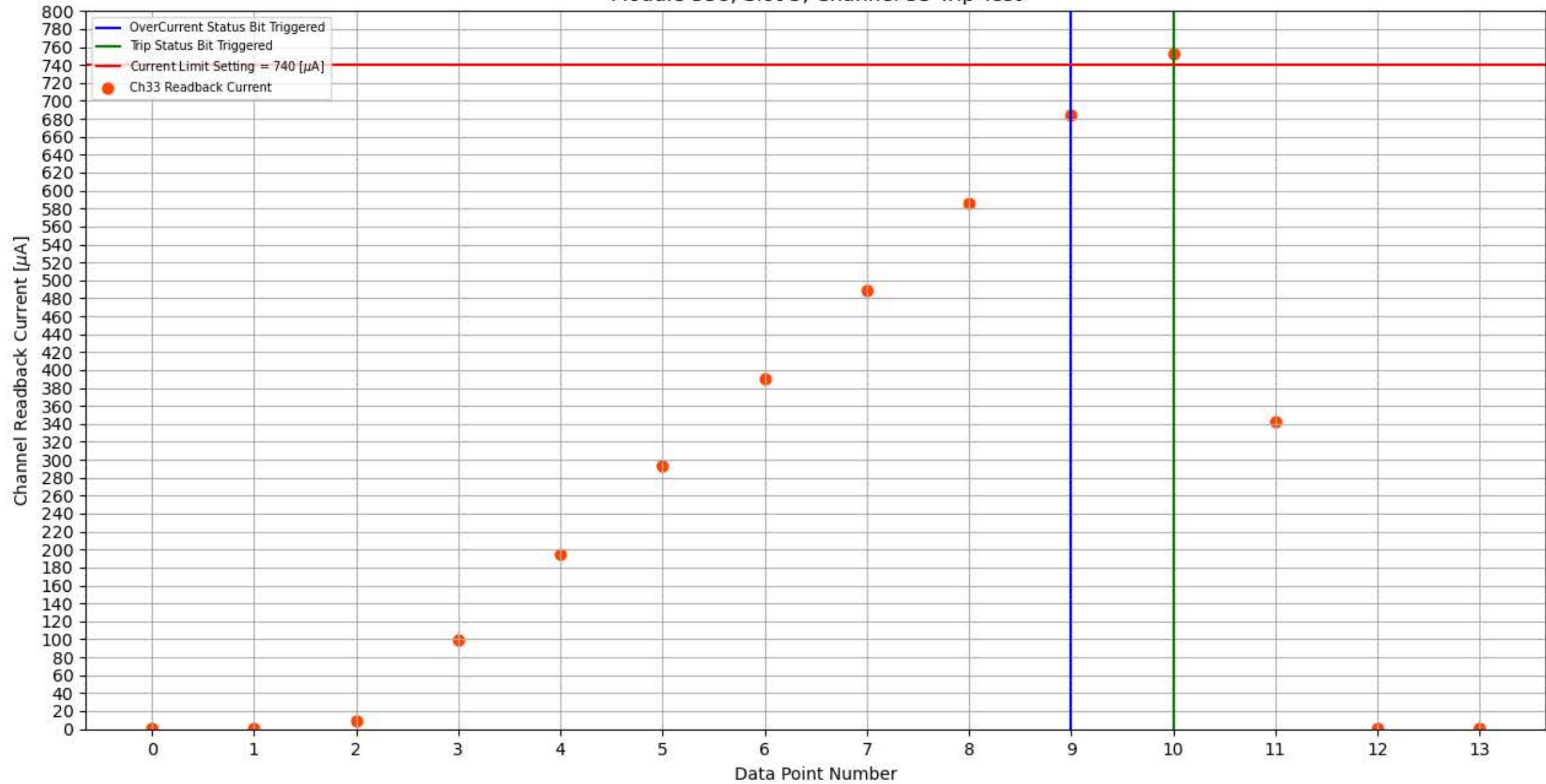
Module 338, Slot 5, Channel 33 Trip Test
