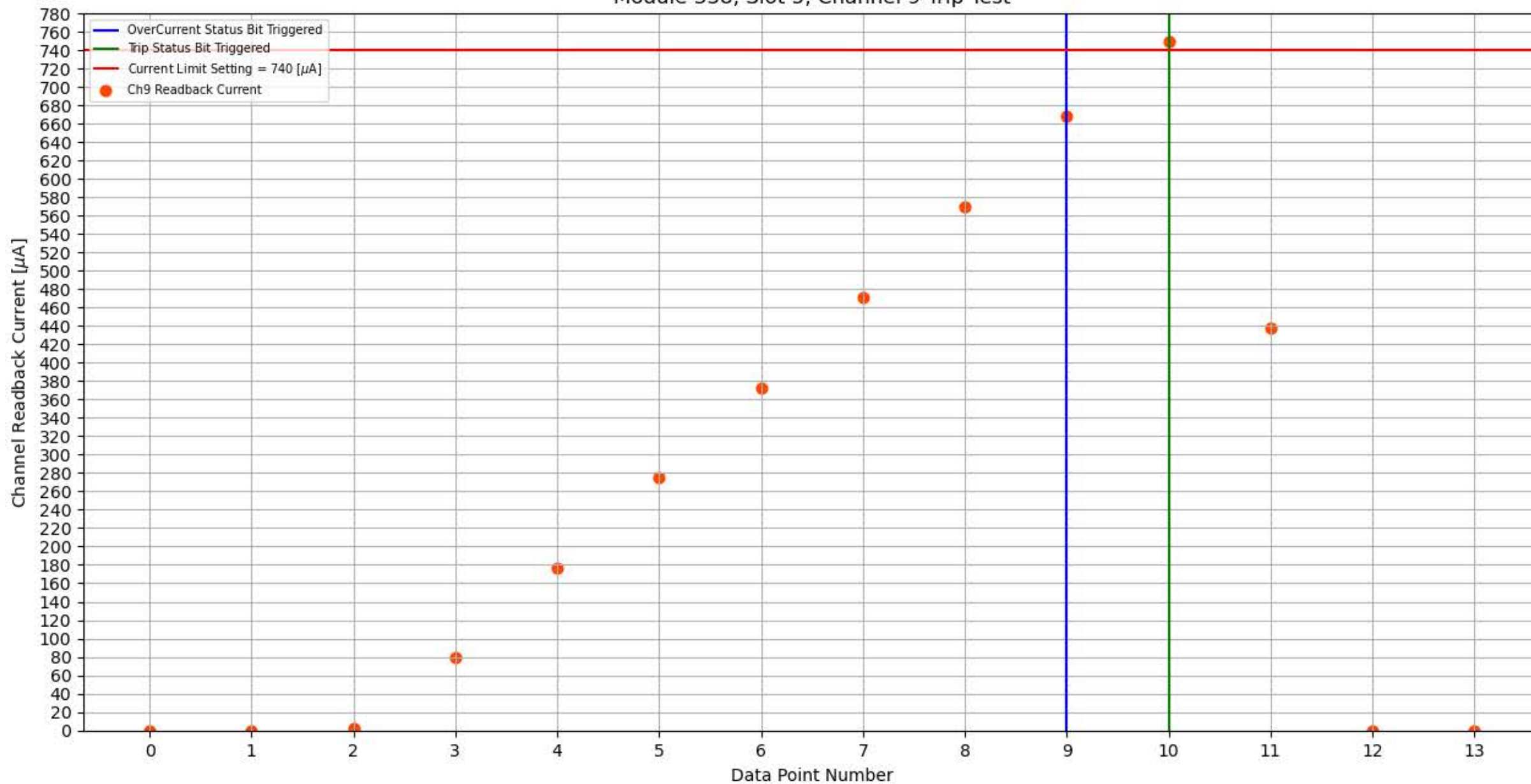
Module 338, Slot 5, Channel 9 Trip Test
