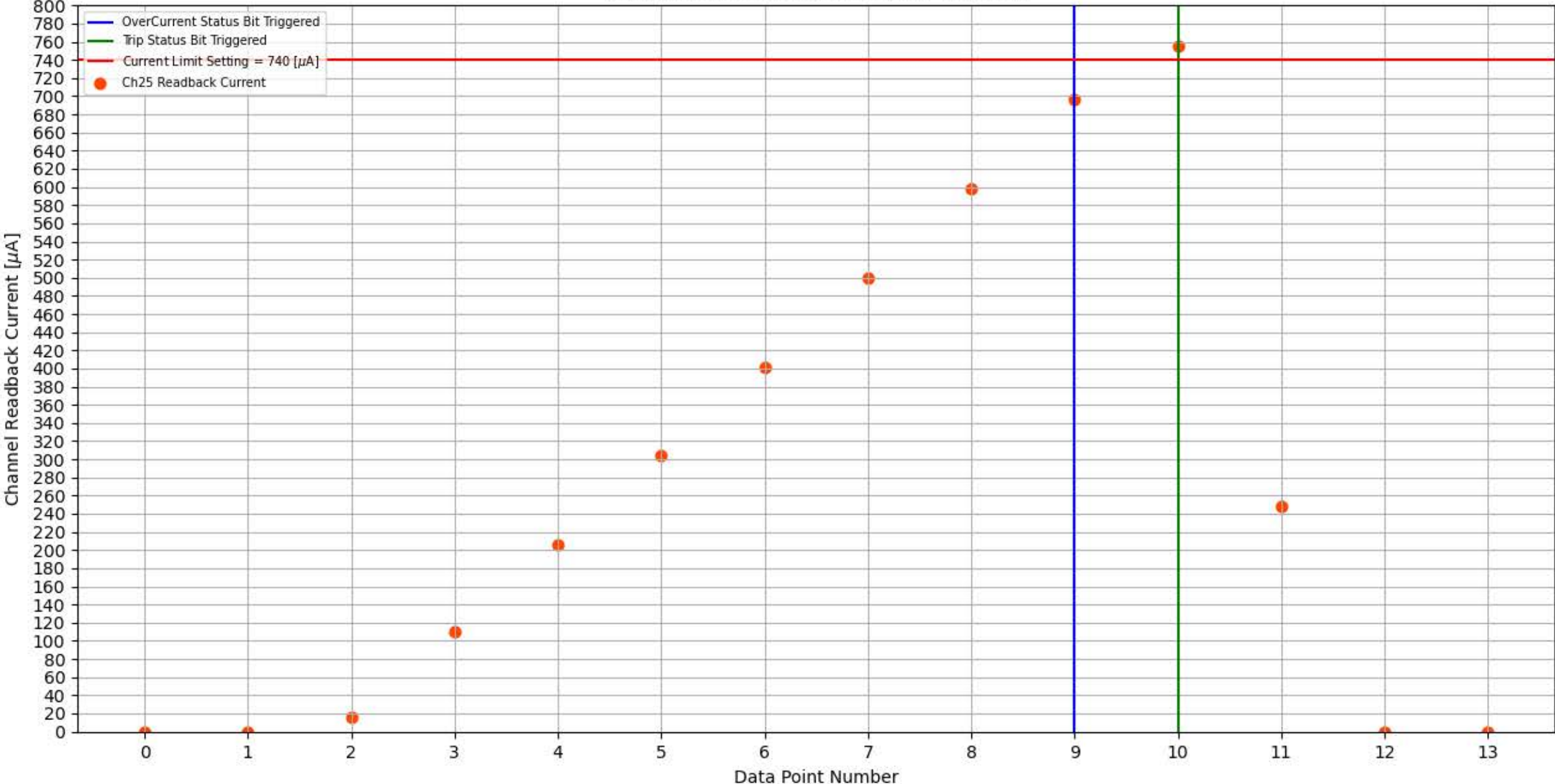
Module 338, Slot 5, Channel 25 Trip Test
