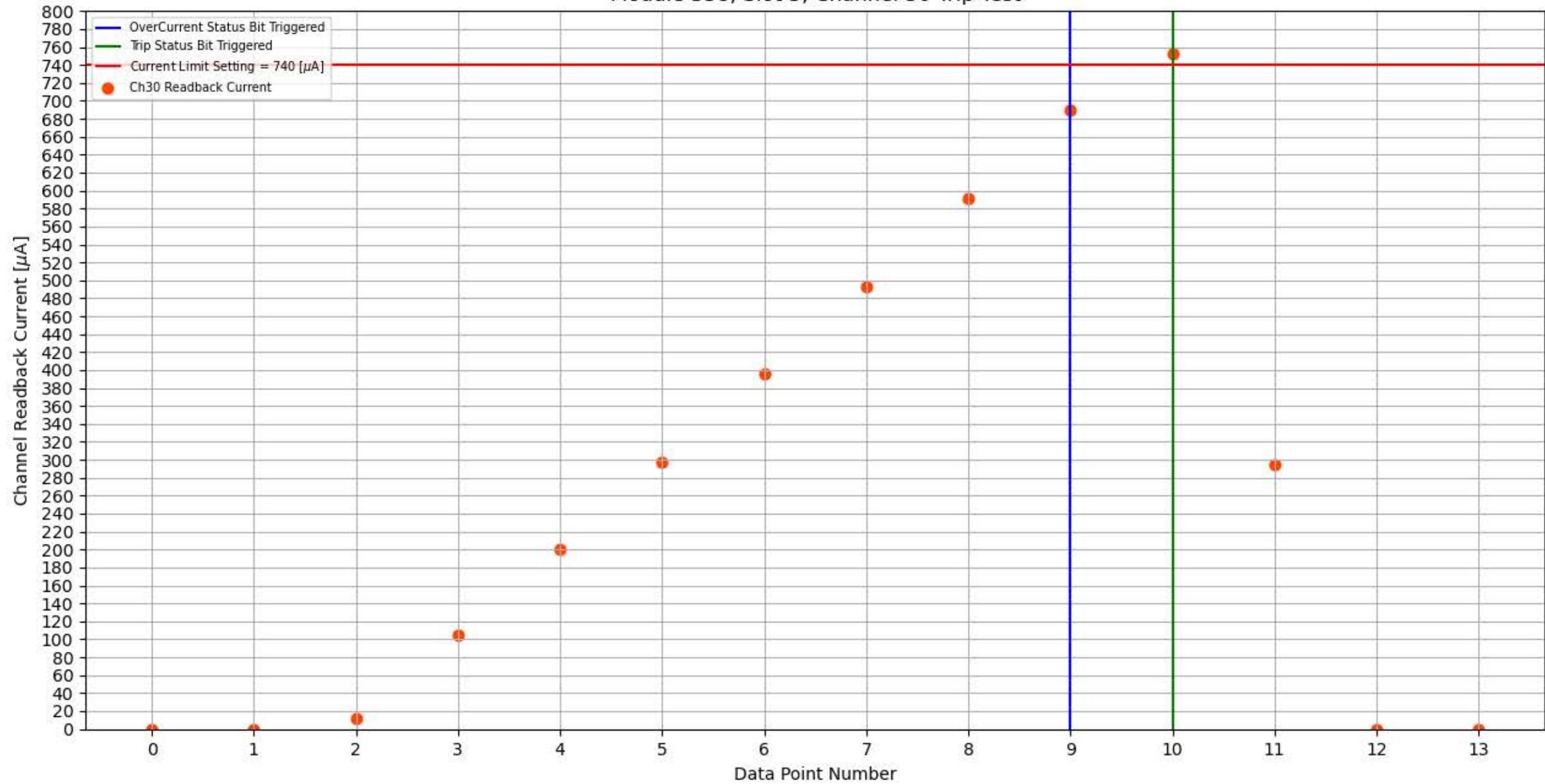
Module 338, Slot 5, Channel 30 Trip Test
