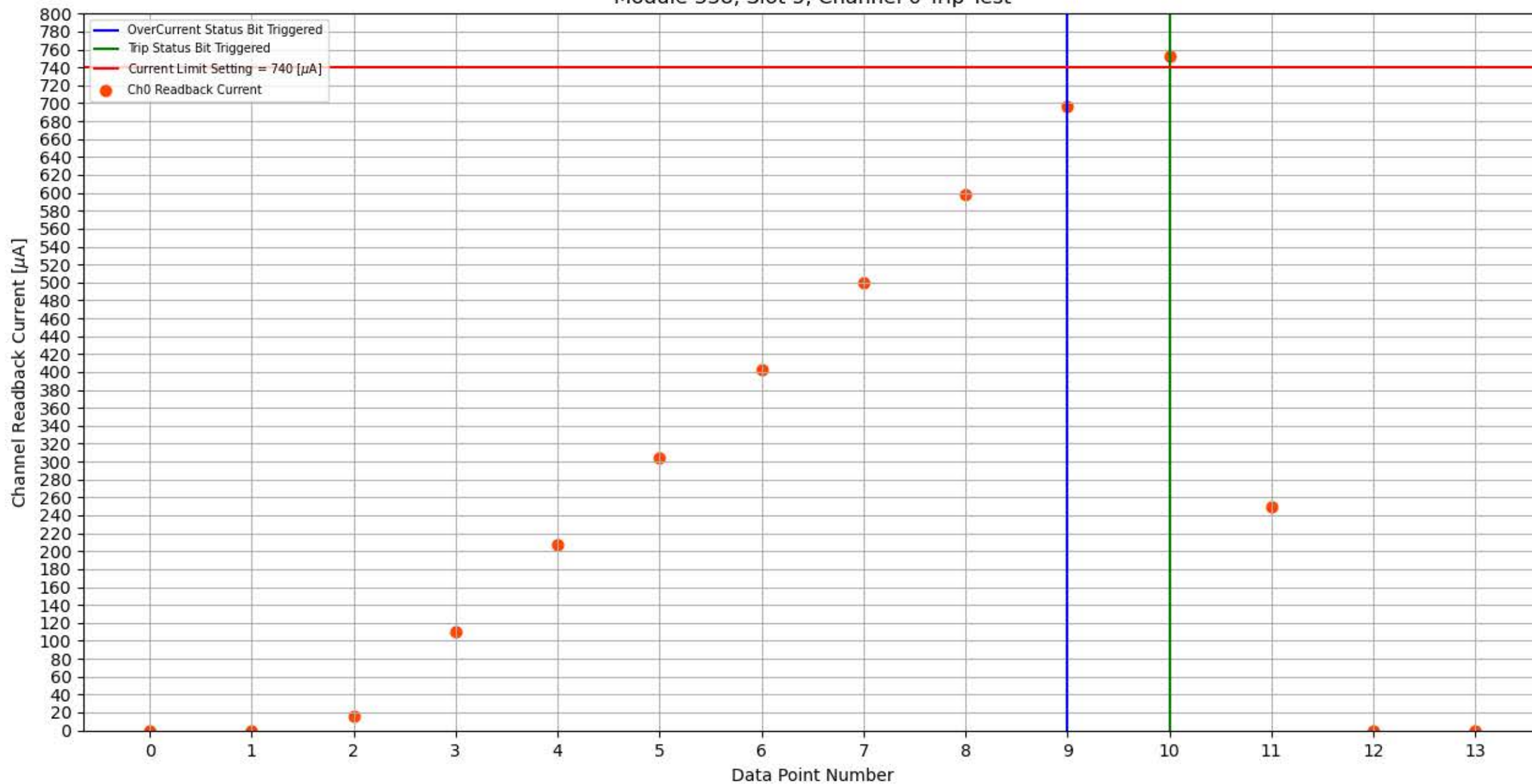
Module 338, Slot 5, Channel 0 Trip Test
